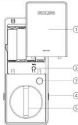
Interior Assembly
