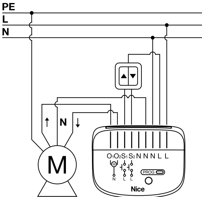
NICE Roll-Control2
