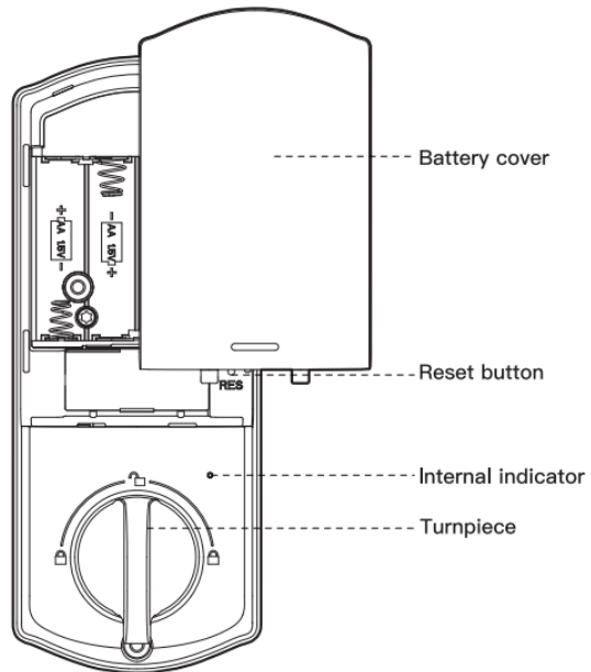
Interior assembly
