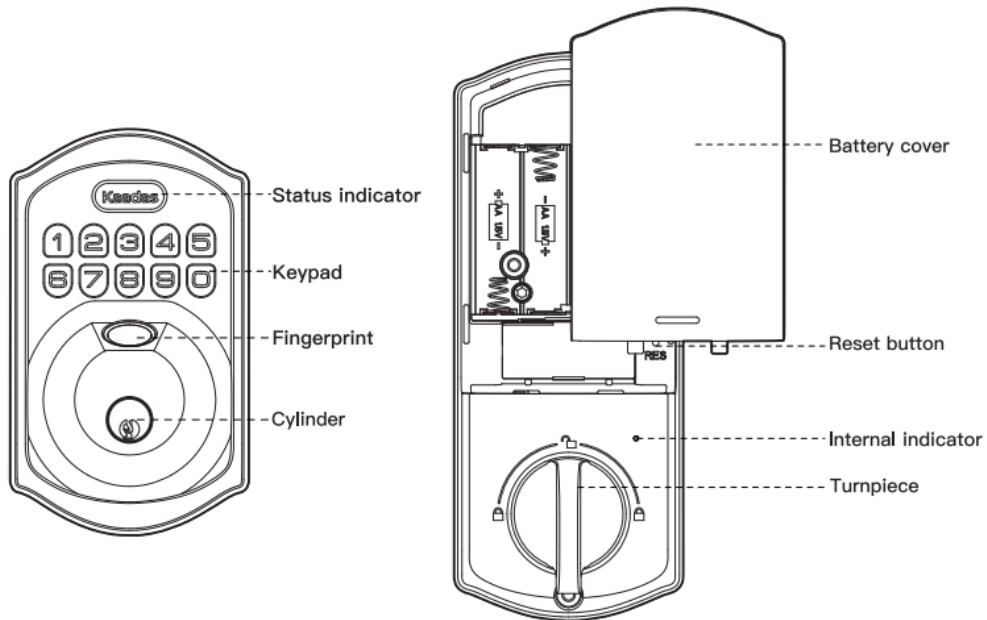
Exterior assembly
