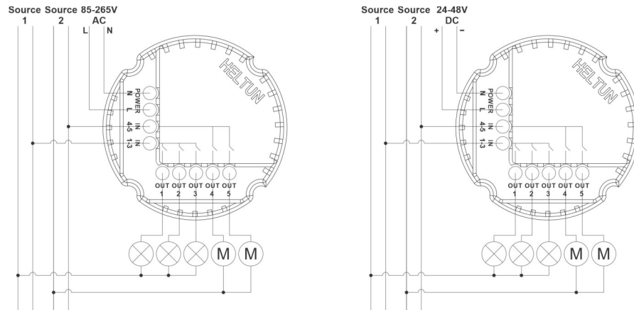
Figure 2: Connection Diagrams
