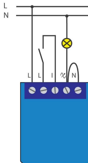
2-wire installation (110 – 240 Vac)
