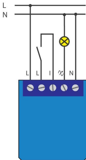
3-wire installation (110 – 240 Vac)
