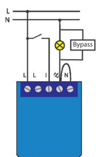
2-wire installation (110 – 240 Vac) With Bypass
