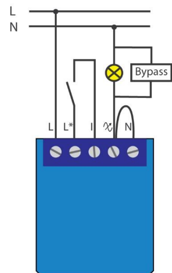
2-wire installation (110 – 240 Vac) With Bypass
