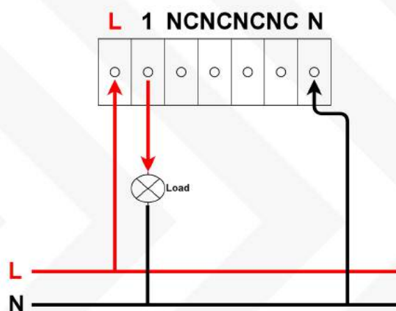
1 Touch Panel Connection
