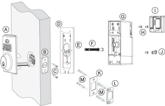
Figure 4: Smart lock installation overview
